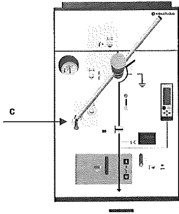
Figure 5.54: End Position of the Lever
