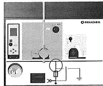
Figure 5.24: Connected Switch-Disconnect
