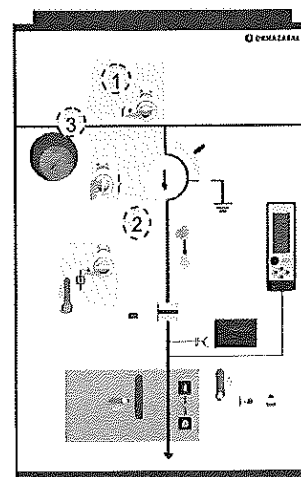
Figure 5.24: Locking in the CGMCOSMOS-V cubicle
