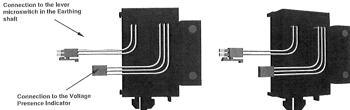
Figure 6.4: ekorSAS connection
