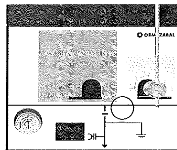
Figure 5.8: Connected Earthing Switch
