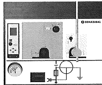
Figure 5.29: Connected Earthing Switch
