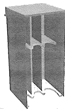
Figure 5.14: Detail of the Base terminal cover box
